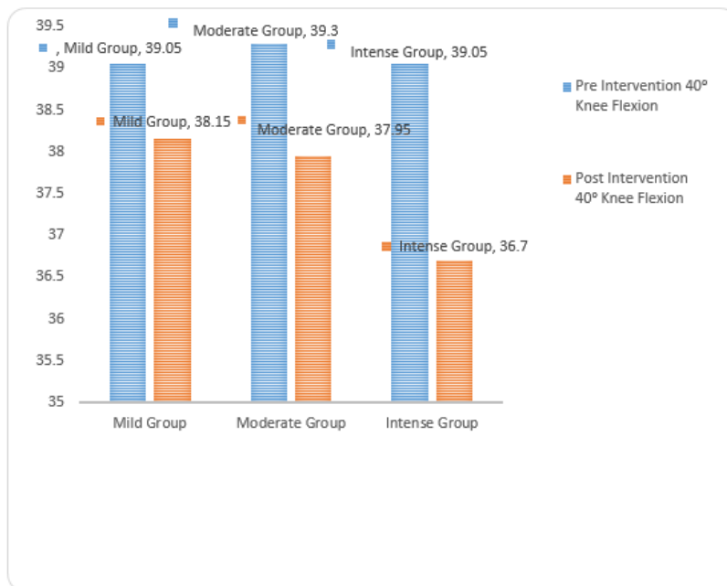
Graph 01: Comparison of Means at 40 degrees of Knee Flexion before & after Physical Activity
