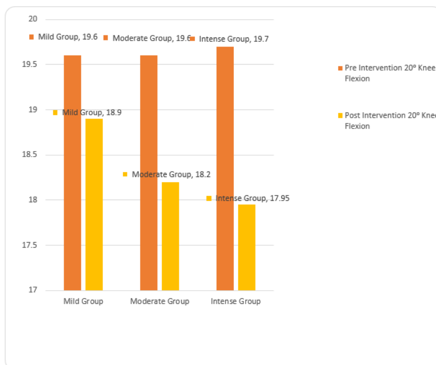
Graph 02: Comparison of Means at 20 degrees of Knee Flexion before & after Physical Activity
