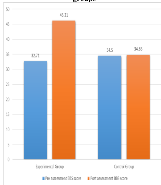
Figure 2: Cluster Bar Chart showing Berg Balance Scale Score of pre and post-treatment values of both groups
